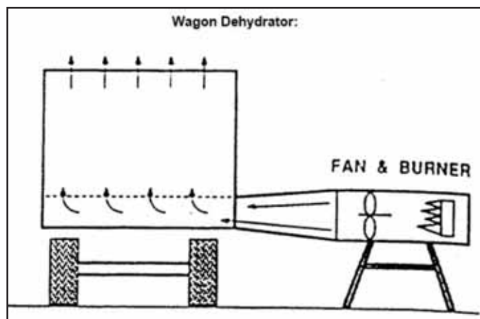
Figure 31 Heat-assisted Batch Dryer
