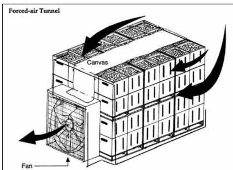
Figure 21 Small-scale Model of a Portable Forced Air Cooling Tunnel
