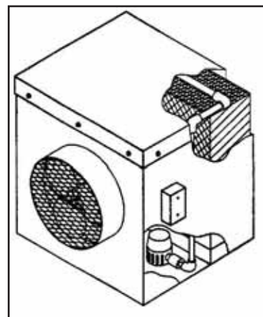
Figure 27 Cut-away View of an Evaporative Cooler with One Pad
