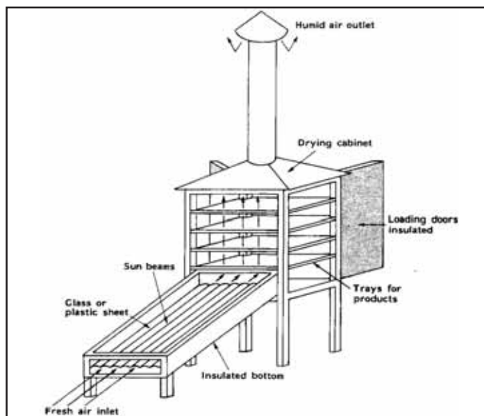
Figure 30 Indirect Solar Dryer
