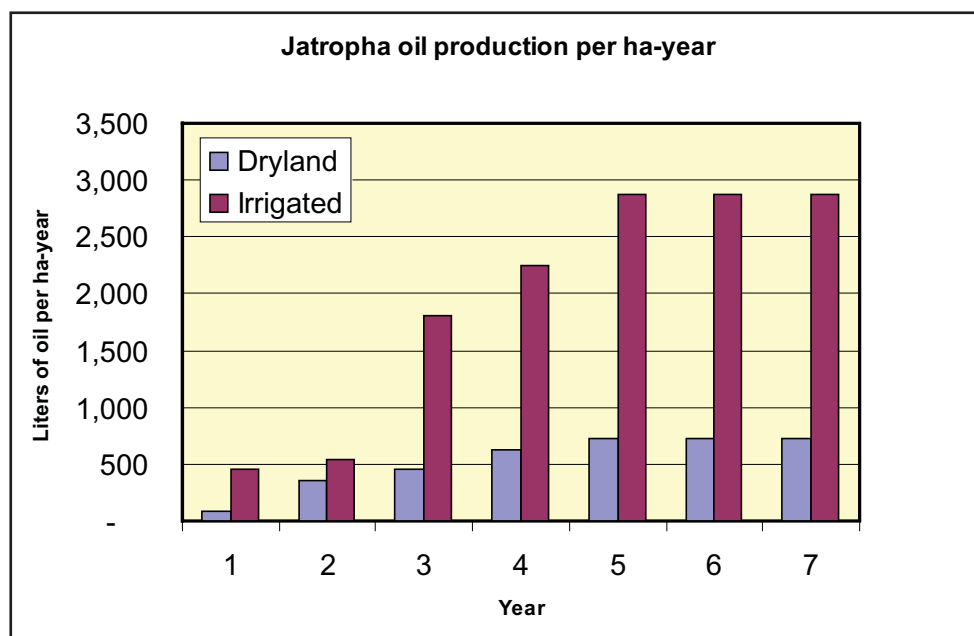
Figure 35 Jatropha Oil Production
