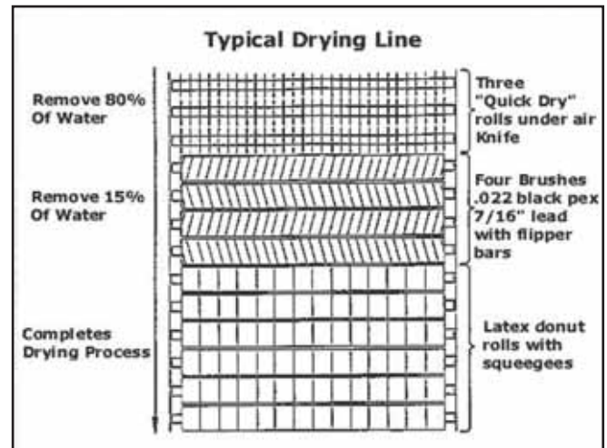
Figure 16 Typical Line Drying
