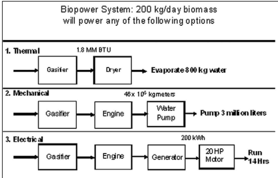
Figure 38 Biomass Gasification System
