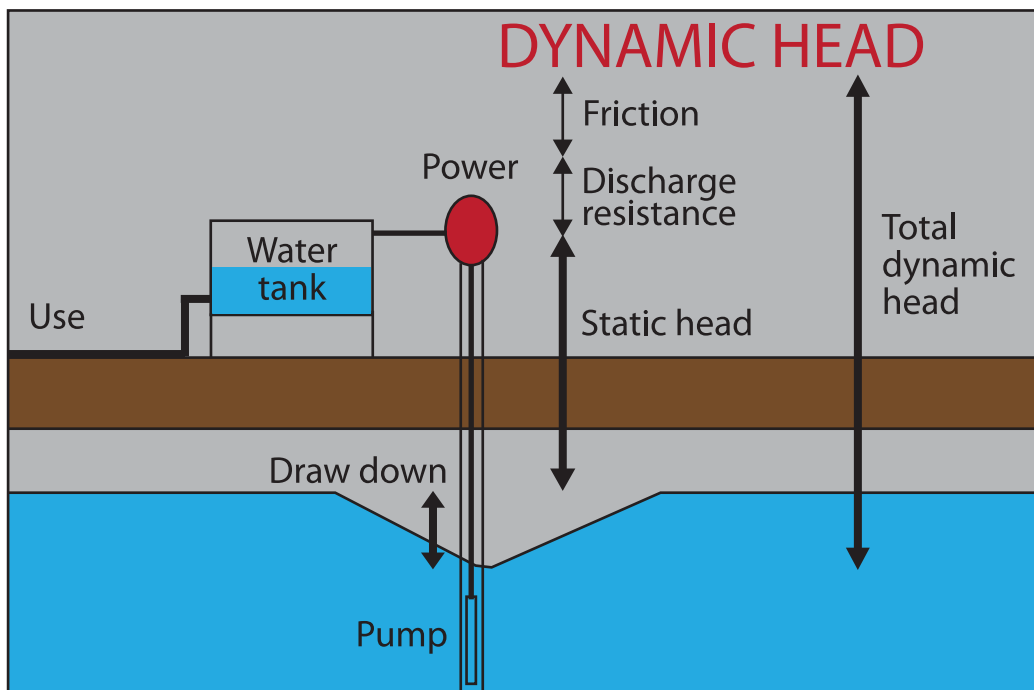
Figure 1 Definition of Dynamic Head for Water Pumping
