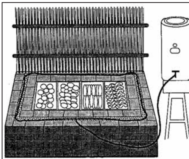
Figure 26 “Zero Energy” Cool Chamber
