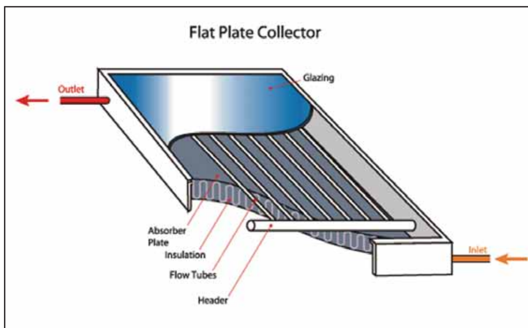
Figure 18 Flat Plate Solar Collector
