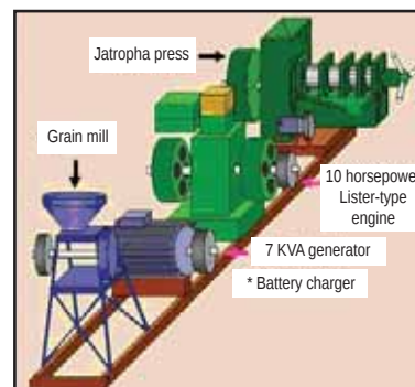
Figure 37 Multi-function Platform Structure
