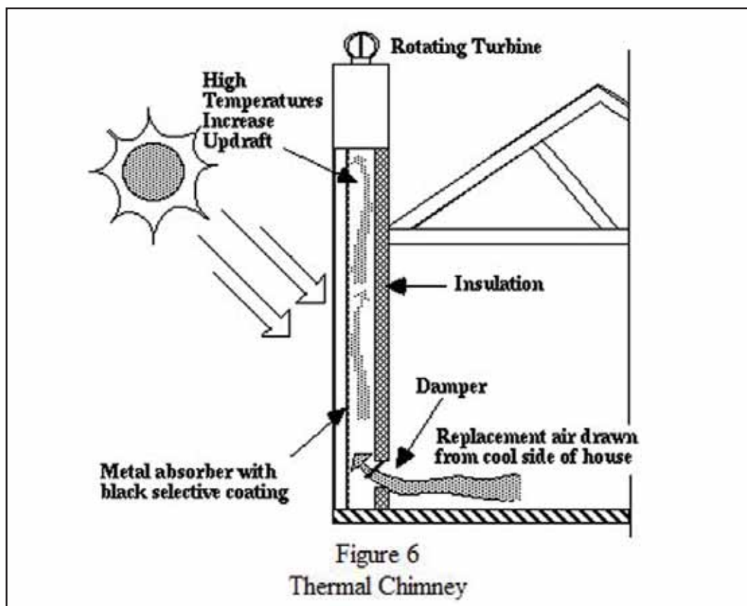
Figure 12 Use of a Thermal Chimney for Low-Energy Cooling
