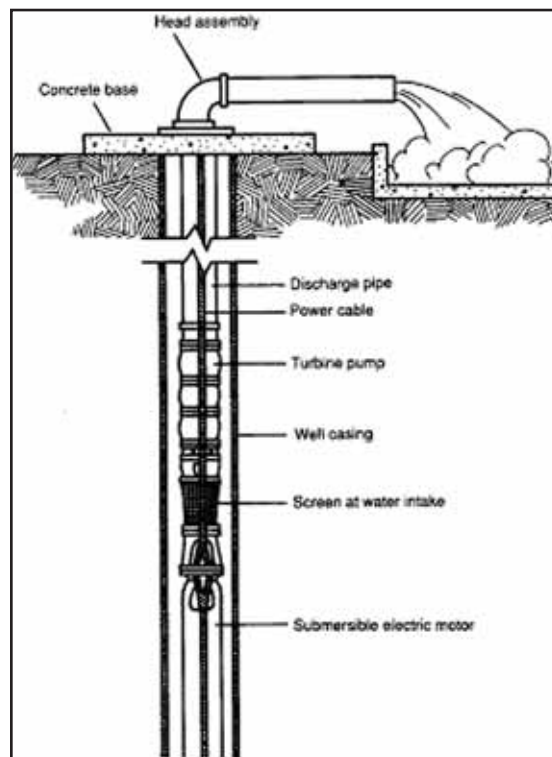
Figure 6 Submersible Electric Pump
